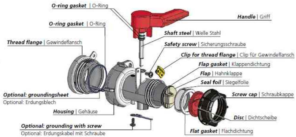
butterfly valve Klappenhahn
