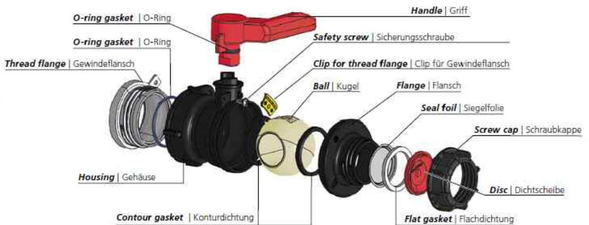
ball valve Kugelhahn
